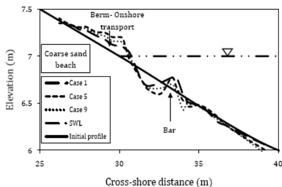
Figure 1: Numerical results for beach face profile changes on the coarse sand beach for the lower inland watertable (cases 1 ( H = 0.15 m, T = 2 s), 5 ( H = 0.25 m, T = 2 s) and 9 ( H = 0.15 m, T = 4 s), for all cases: GWT = 5.5 m)
